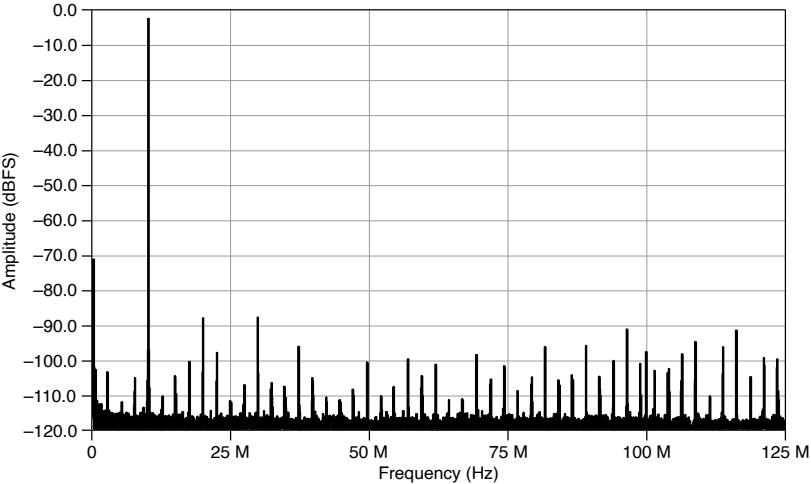
-1 dBFS, Measured
