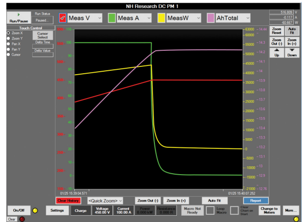
Figure 3 - Chart Recorder
