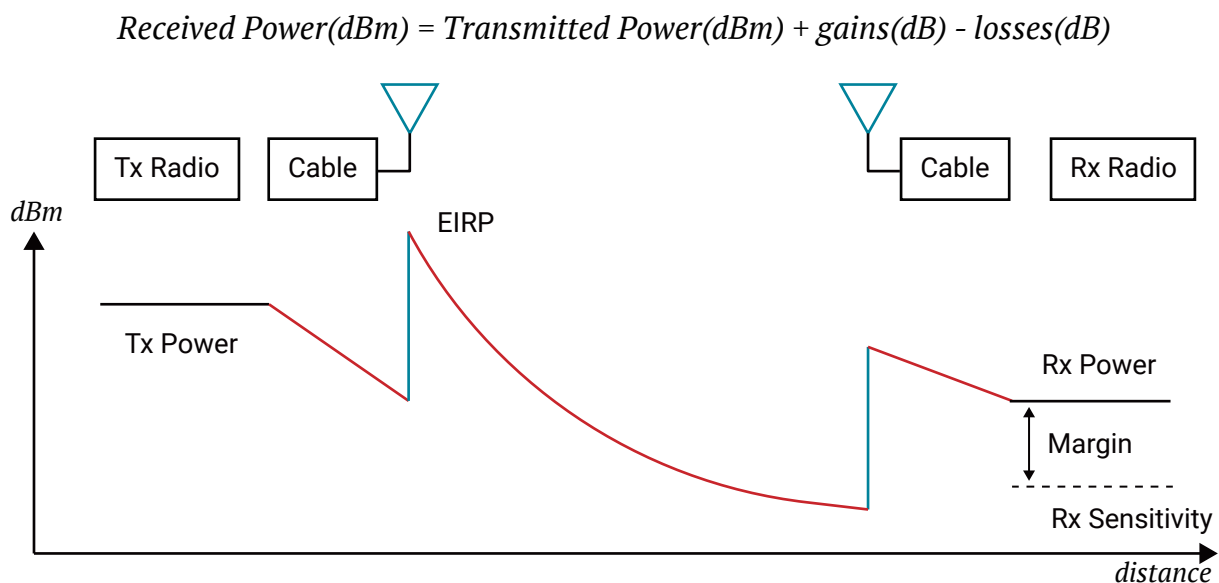
Figure 2. Link Budget Overview
