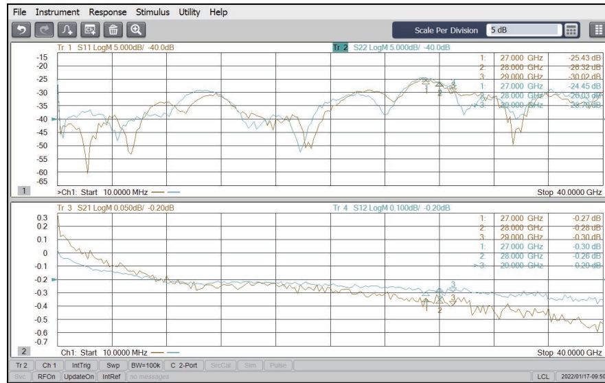
Figure 9. S-Parameter of the Adapter
