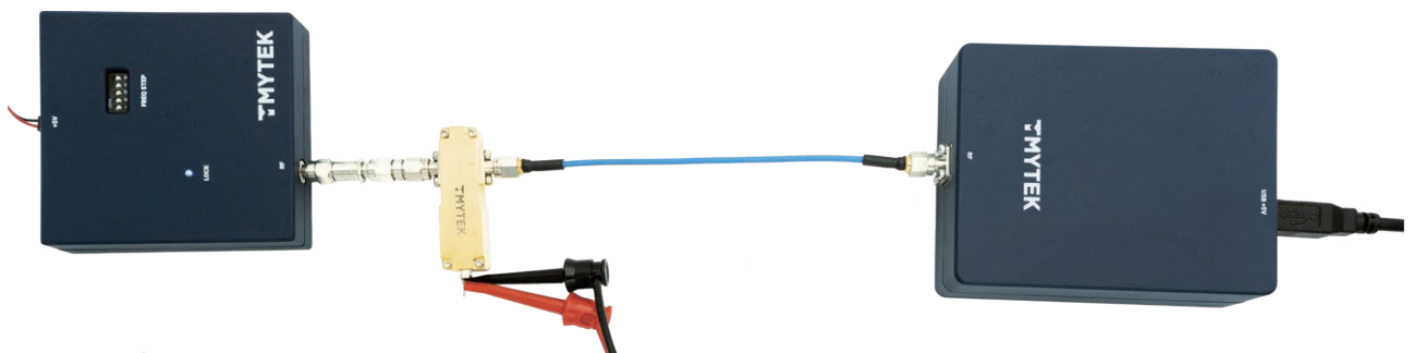
Figure 8. PLO + Attenuator + Adapter + Amplifier + Cable
