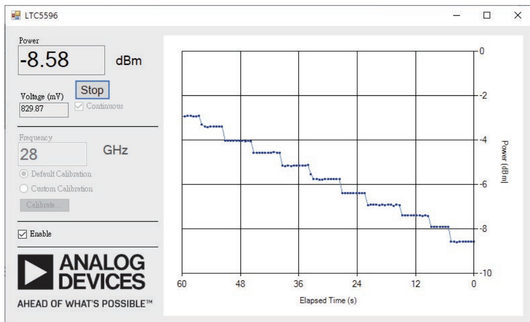
Figure 12. Measured Power from LTC5596
