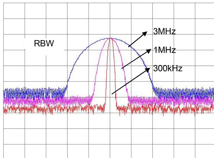
Figure 5-1 Impact of Resolution Bandwidth on Measurement Results
