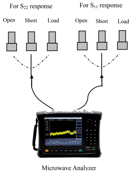
Figure 4-6 Standard piece correction for single port reflection error correction
