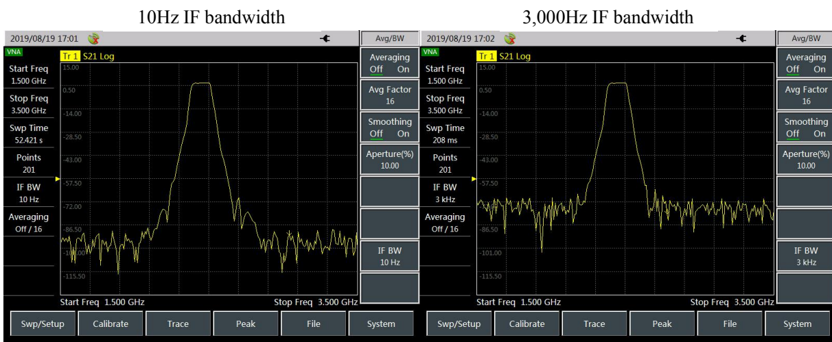
Figure 4-2 Effect of IF Bandwidth on Measurement Results
