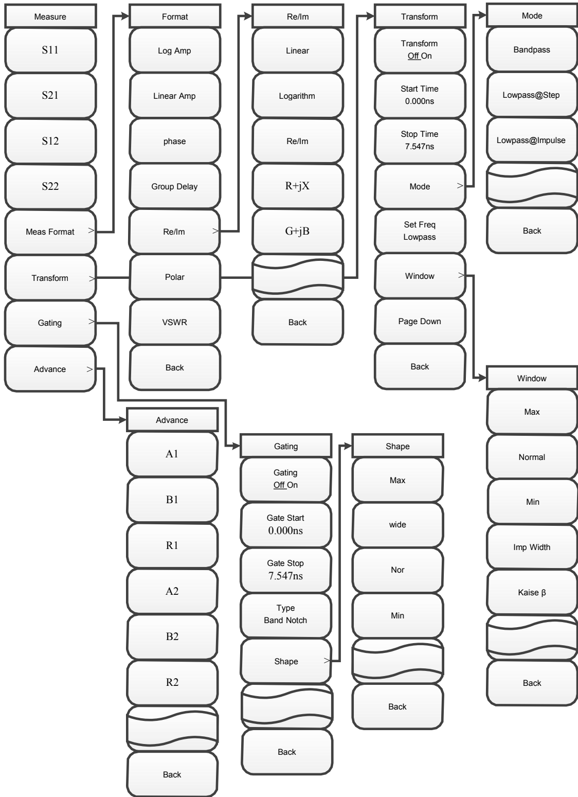
Figure 4-8 Menu structure of measure
