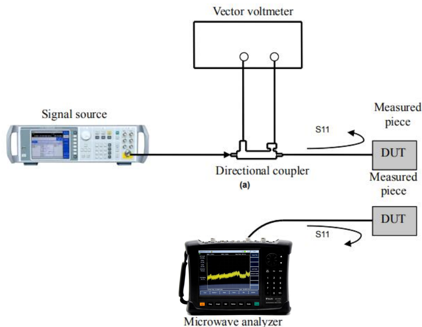
Figure 8-1 Measurement Structure Comparison of Vector voltmeter and S5105D/E/F Vector Voltage Measurement Mode
