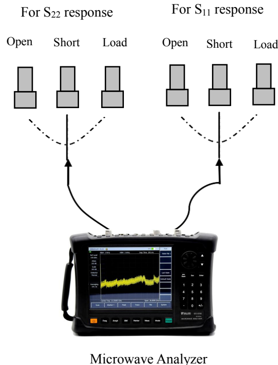
Figure 4-3 Standard piece connection for reflection measurement response error correction
