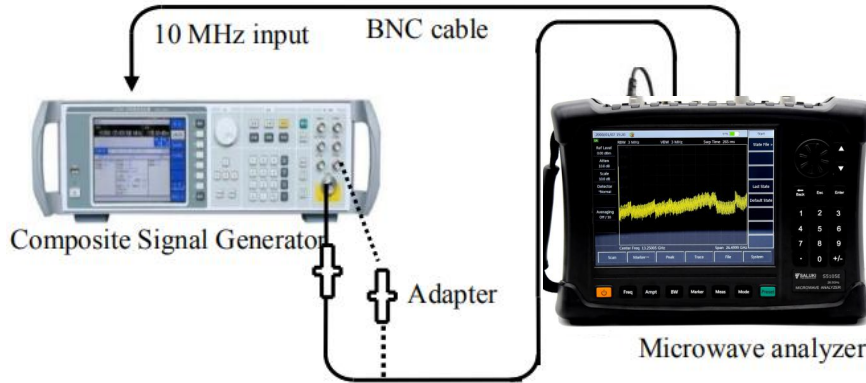
Figure5-33 Frequency Span Test Block Diagram
