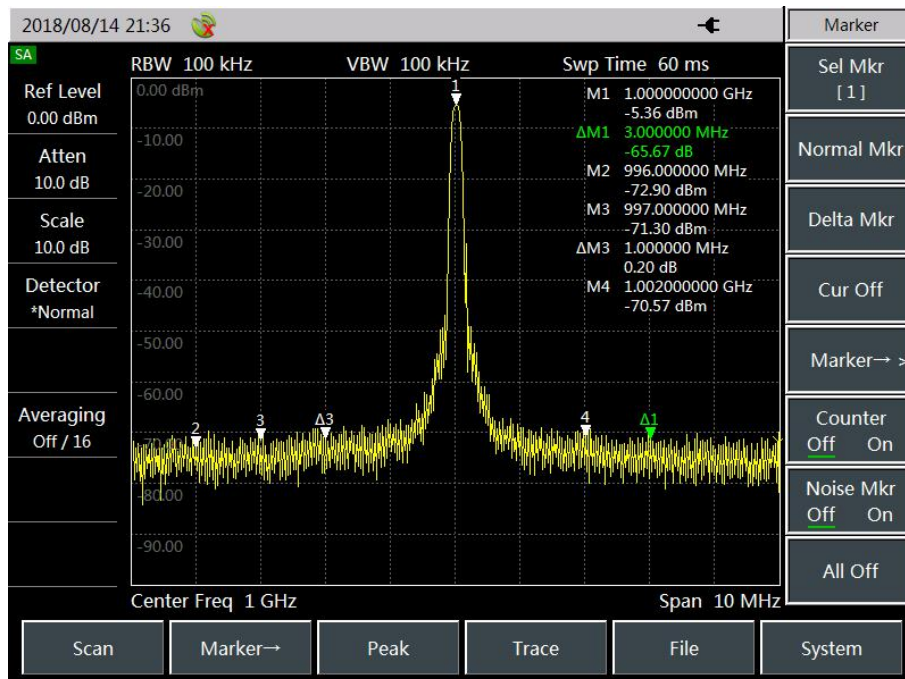
Figure 5-6 Marker Function
