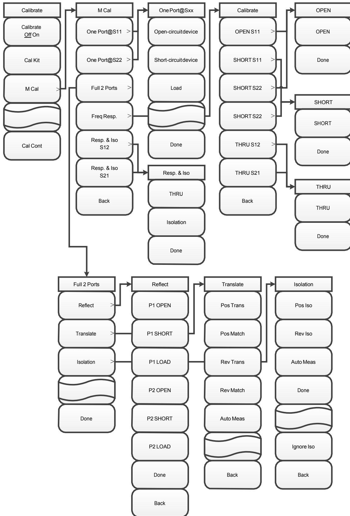
Figure 4-12 Menu structure of calibration
