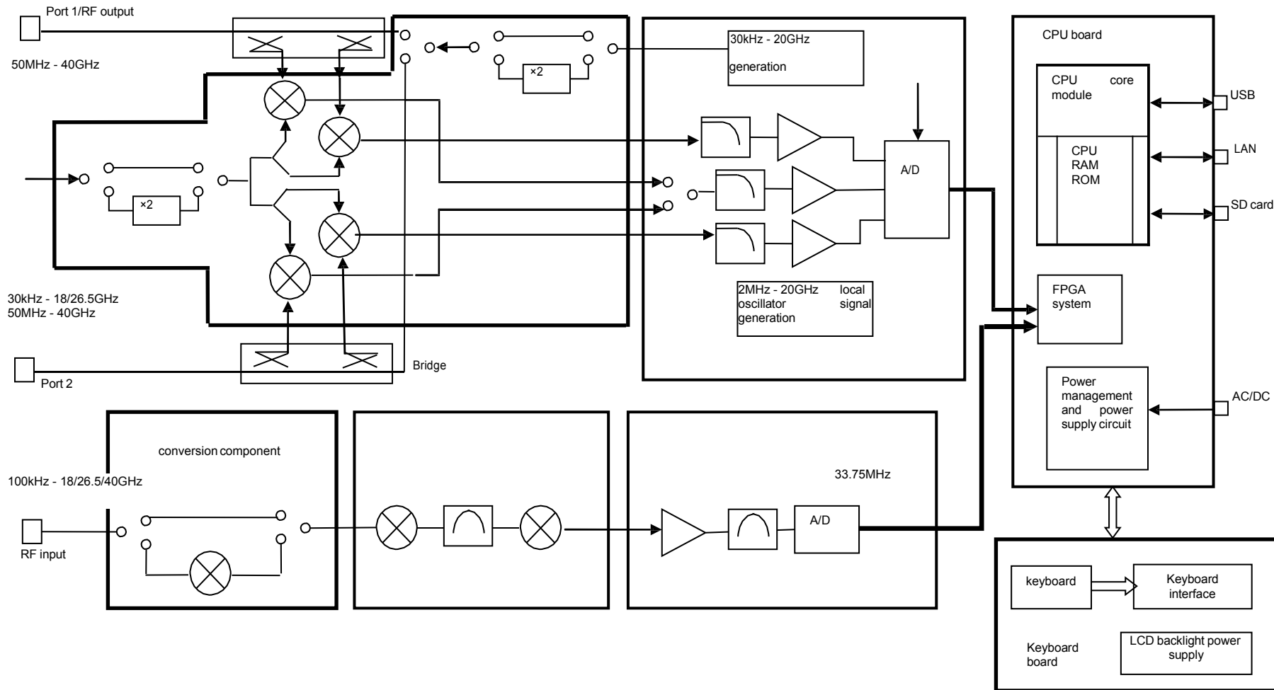
Figure 10-1 Block Diagram of the S5105D/E/F microwave analyzer
