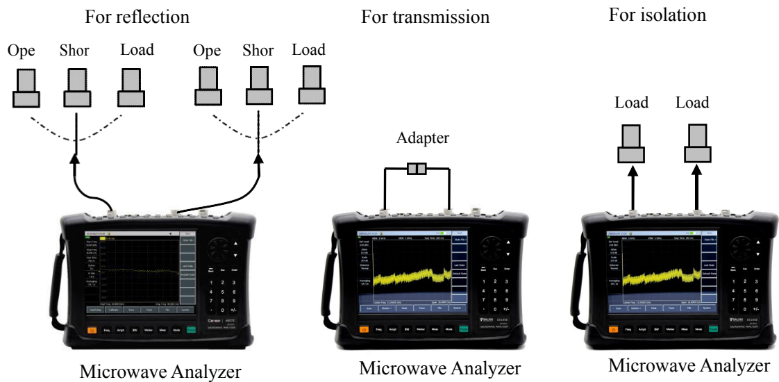
Figure 4-7 Standard piece correction for Full 2 ports error correction
