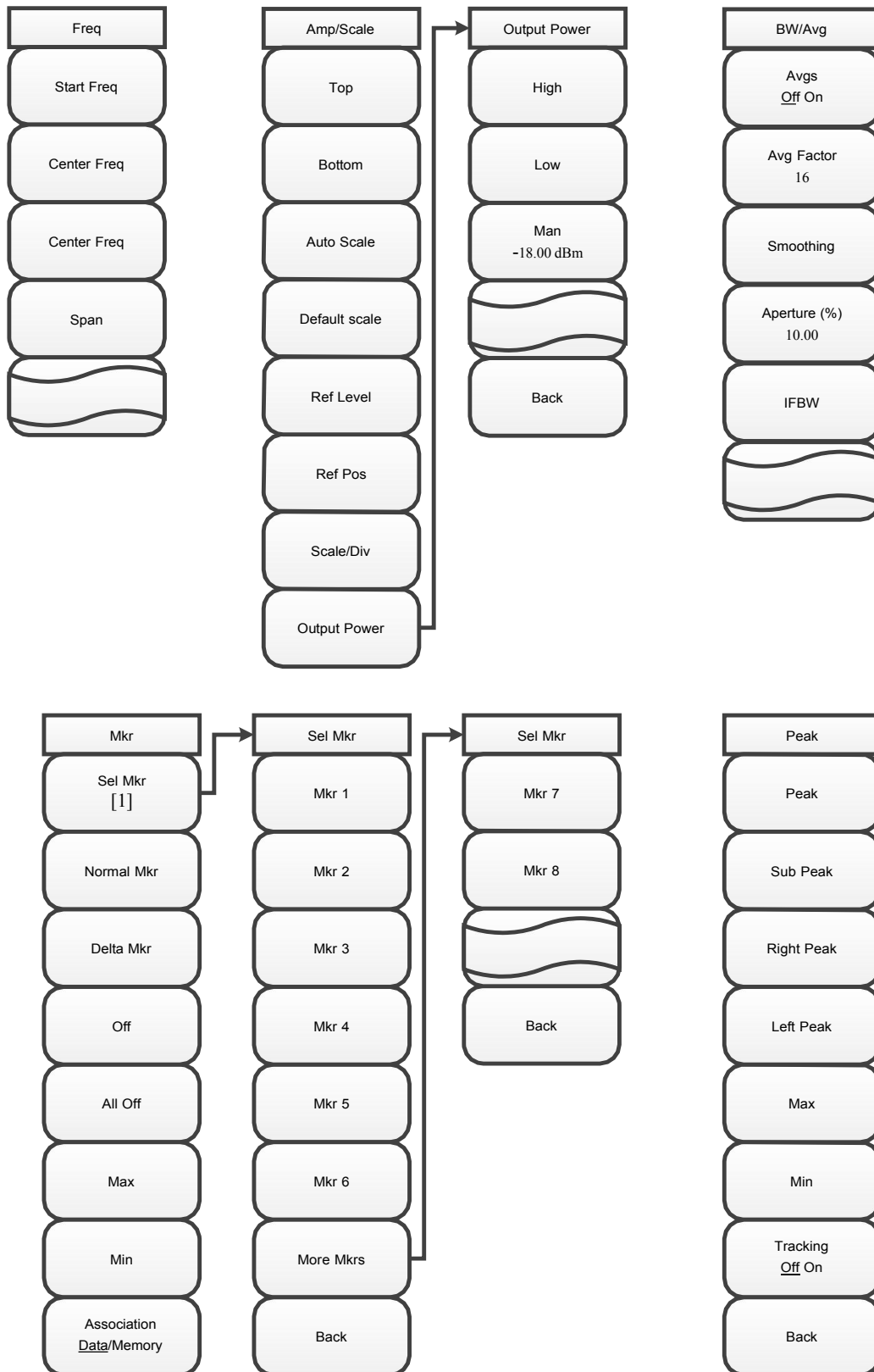
Figure 4-9 Menu structure of frequency, amplitude/scale, bandwidth/averaging, marker and peak
