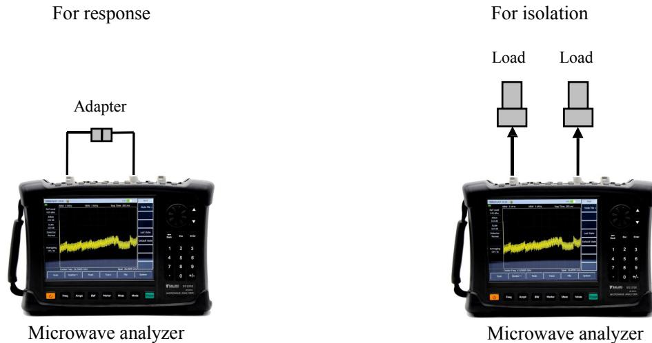
Figure 4-5 Standard piece connection for transmission measurement response and isolation error correction
