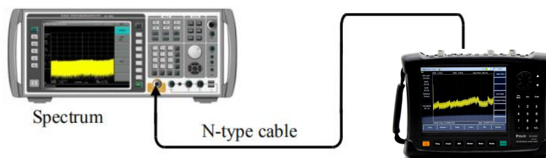
Figure 4-13 Test block diagram of frequency range and frequency accuracy
