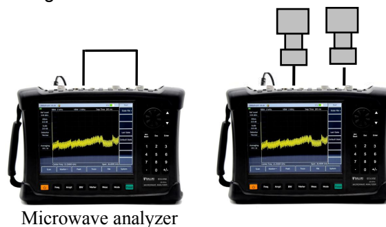
Figure 4-16 Test block diagram of dynamic range and transmission tracking
