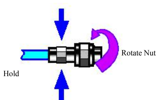
Figure 3 -2 Connection method
