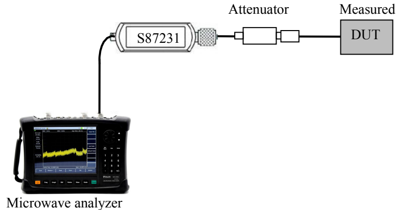
Figure 9-1 Measurement Structure of S5105D/E/F USB Power Meter Mode
